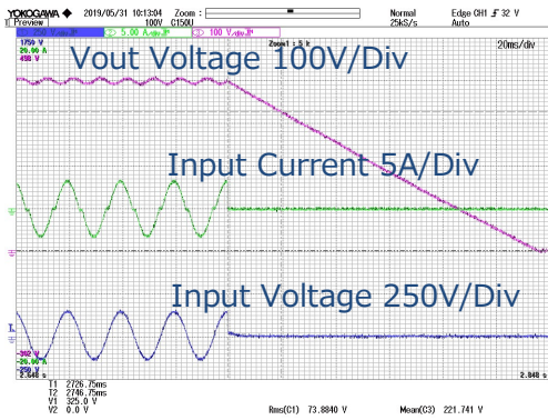
Figure 20. Hold time
