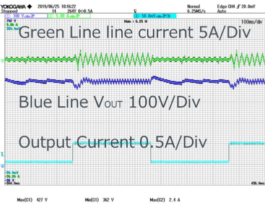
Figure 24. Load Transient V_{IN} = 264\text{ V}_{AC}
