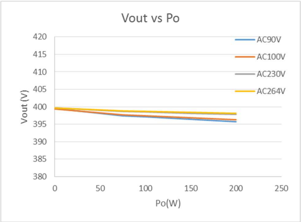
Figure 8. Load Regulation ( P_o vs V_{OUT} )
