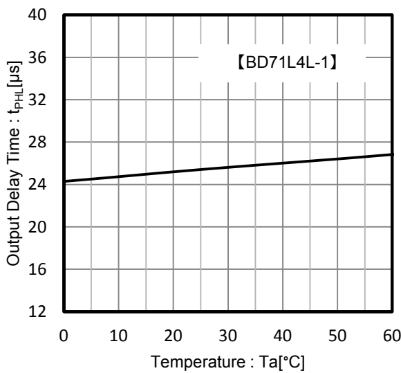
Figure 10. Output Delay Time (t PHL ) V_{DD}=V_{DET}-0.5V to V_{DET}+0.5V V_{DD}=3.55V to 4.55V
