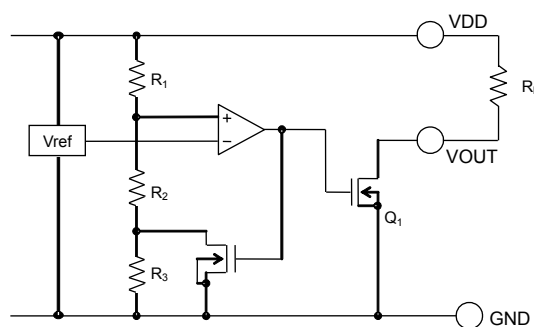
Figure 14. Internal Block Diagram
