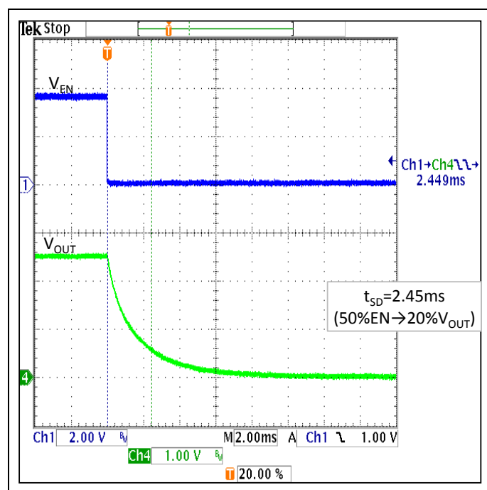
Figure 37. Shutdown ( V_{IN}=3.6V , V_{OUT}=2.5V , I_{OUT}=0mA , EN=V_{IN} \rightarrow 0 )
