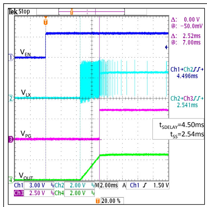
Figure 35. Startup ( V_{IN}=3.6V , V_{OUT}=2.5V , I_{OUT}=0mA , EN=0 \rightarrow V_{IN} )
