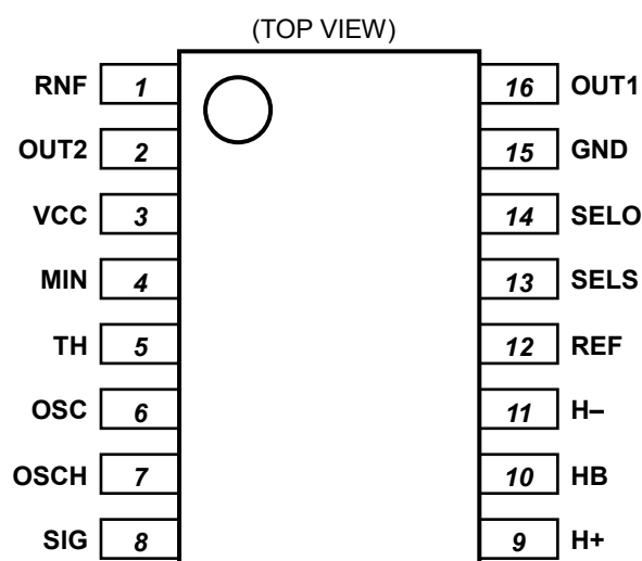
Figure 1. Pin Configuration
