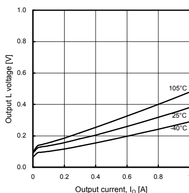
Figure 5. Output L Voltage (Temperature Characteristics)
