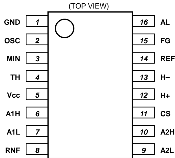
Fig.1 Pin configuration
