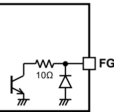
5) Speed pulse signal output terminal
