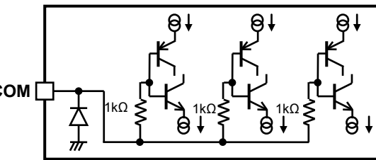
6) Motor coil midpoint input terminal
