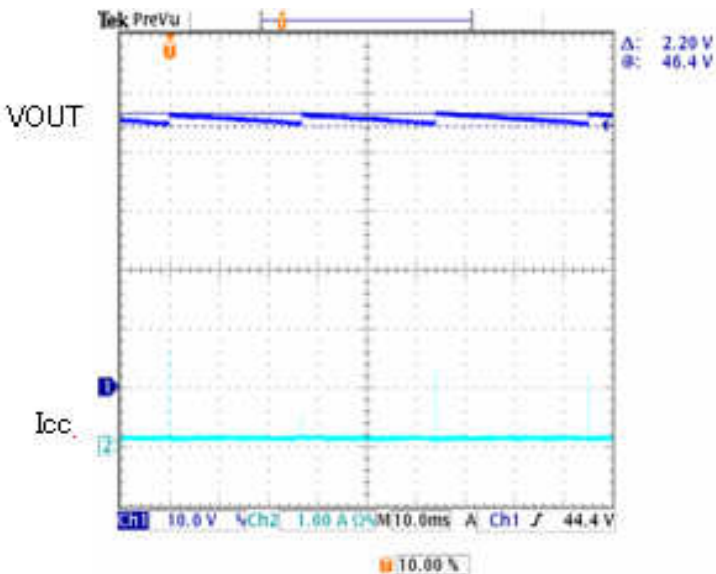
Figure 26. VOUT@OVP(LED OPEN)
