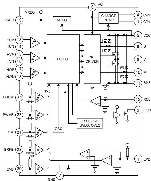
Figure 3. Block Diagram
