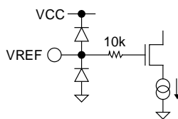
Figure 45. VREF
