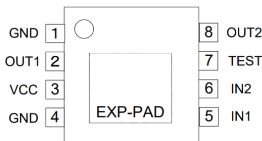
Figure 7. Pin configuration
