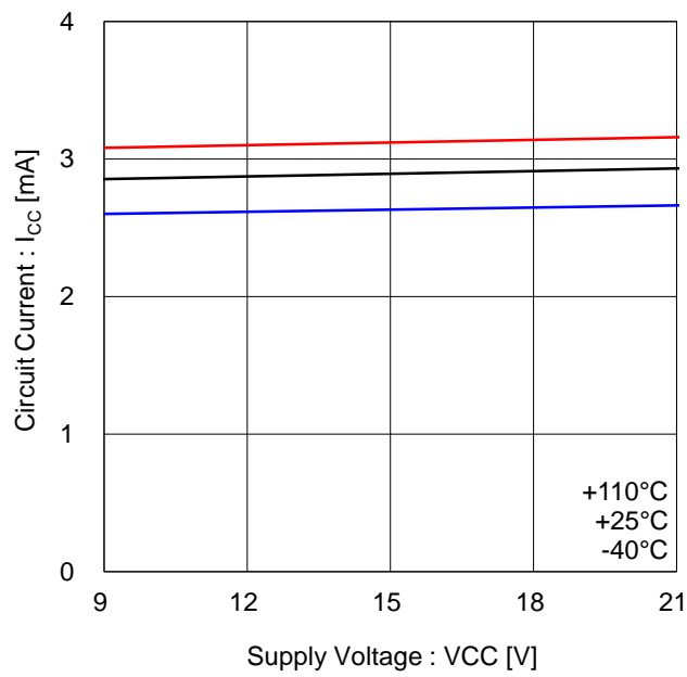
Figure 7. Quiescence Current
