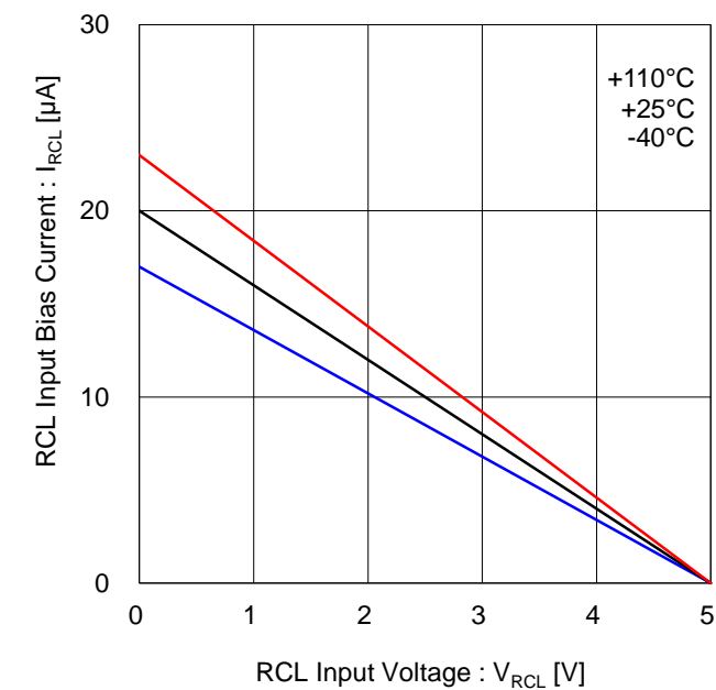
Figure 21. RCL Input Bias Current
