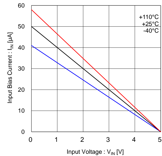
Figure 19. Input Bias Current (CCW, FIB)
