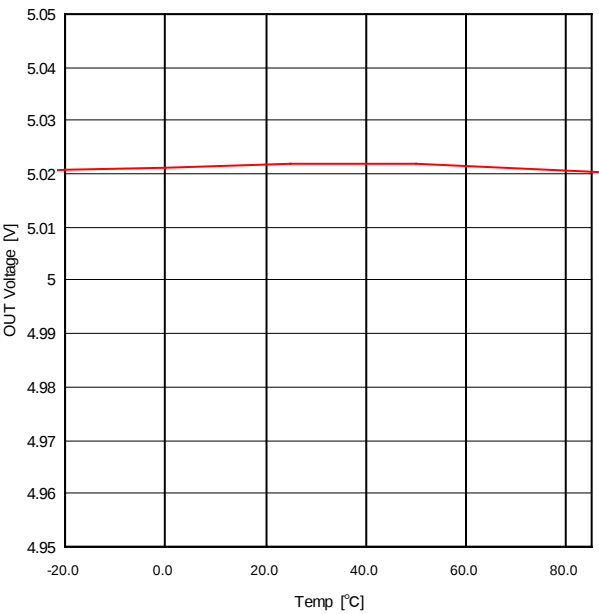
Figure 3. OUT Voltage [V] vs. Temp. [°C] (ILIM=27k Ω)
