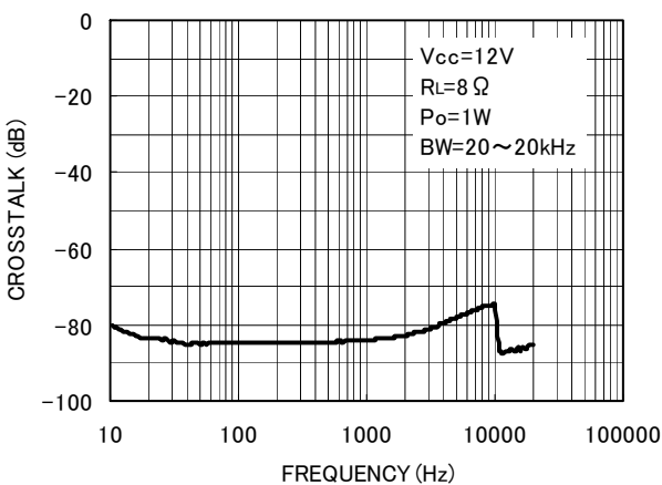
Fig. 4 Crosstalk - Frequency
