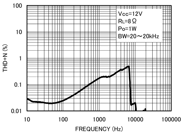
Fig. 2 THD+N — Frequency
