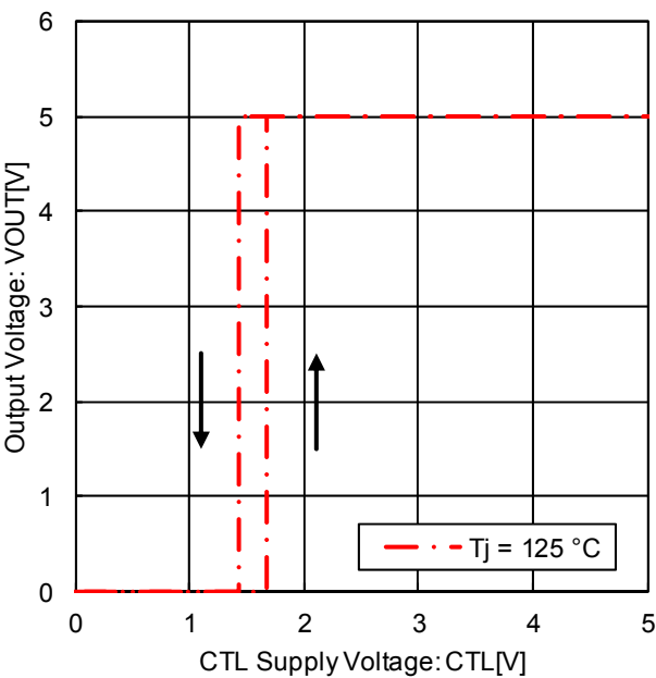
Figure 38. CTL ON / OFF Mode Voltage ( T_j = 125\text{ }^{\circ}\text{C} )
