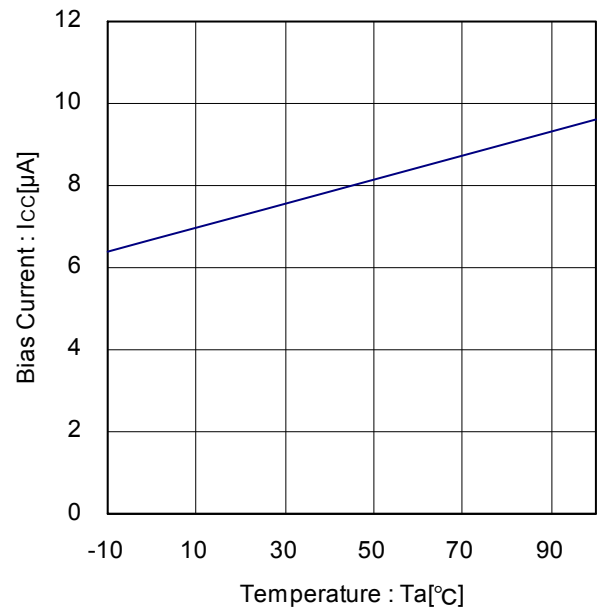
Figure 5. Temperature - Bias Current
