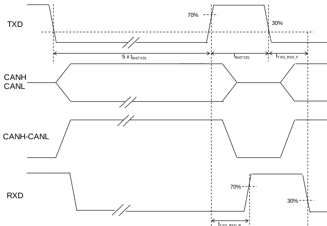
Figure 8. Propagation Delay from TXD to RXD
