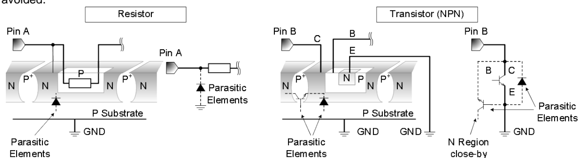
Figure 101. Example of monolithic IC structure
