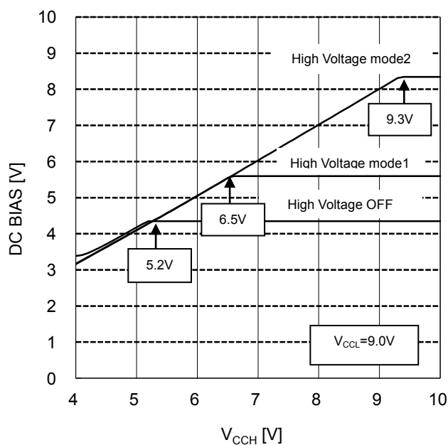
Figure 17. V_{CC} vs DC Bias
