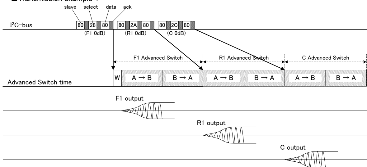
Figure 26. Multi-blocks data transmission timing
