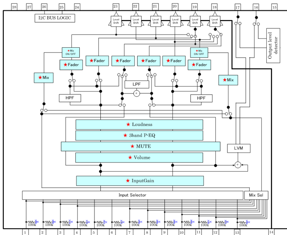
Figure 3. Block Diagram
