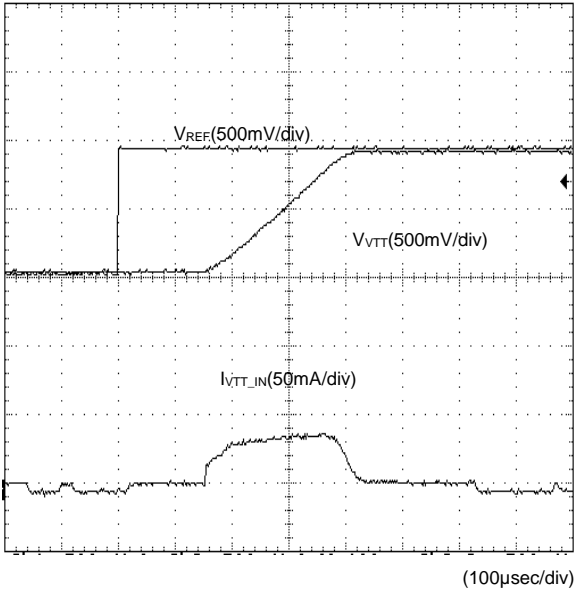
Figure 8. Soft Start
