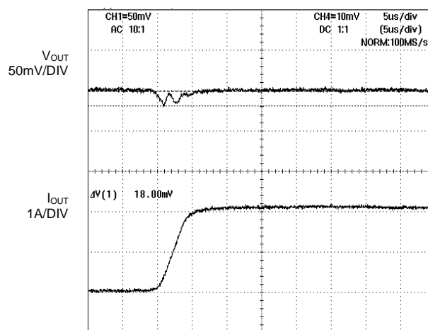
Figure 12. Transient Response (Rise) 47μ MLCC+30mΩ
