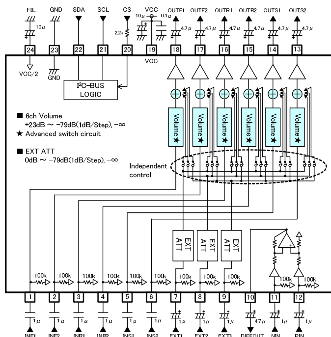
Figure 1. Application Circuit
