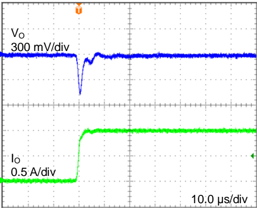
Figure 6. Transient Response (1 mA→1000 mA, Ta = +125 °C)
