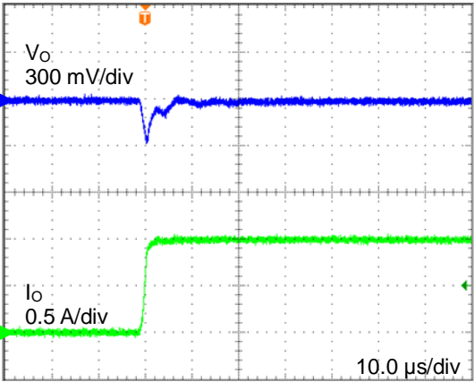
Figure 4. Transient Response (1 mA→1000 mA, Ta = -40 °C)
