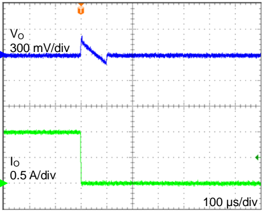
Figure 7. Transient Response (1000 mA→1 mA, Ta = -40 °C)
