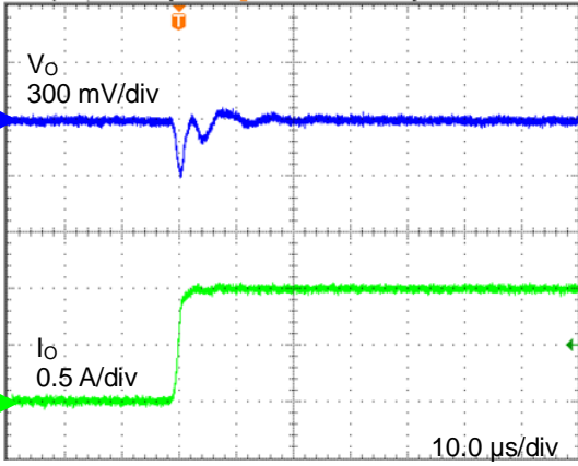
Figure 5. Transient Response (1 mA→1000 mA, Ta = +25 °C)
