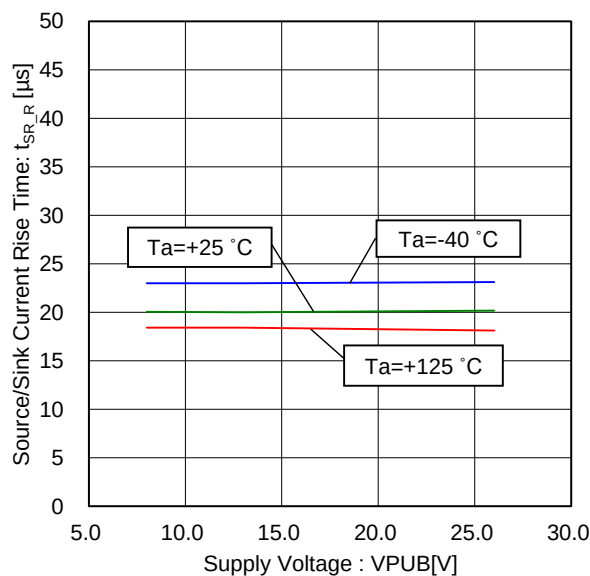
Figure 115. Source/Sink Current Rise Time vs Supply Voltage (FSQ="0", FSQZ/A/B="0", 10 mA Setting, Load Resistance=100 \Omega )
