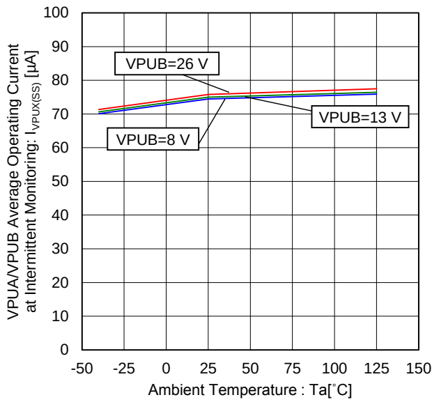
Figure 26. VPUA/VPUB Average Operating Current at Intermittent Monitoring vs Ambient Temperature (Monitoring Period: 50 ms, Strobe Time: 125 \mu\text{s} , Source/Sink Current Setting: 1 mA)
