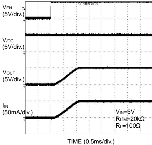
Figure 38. Output Rise Characteristic (BD2242G)
