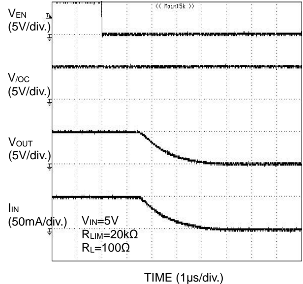
Figure 39. Output Fall Characteristic (BD2242G)
