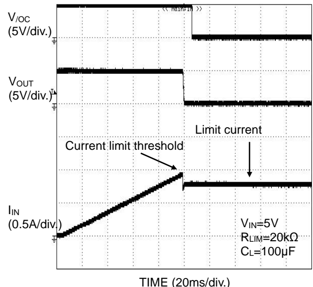
Figure 41. Over Current Response Ramped Load
