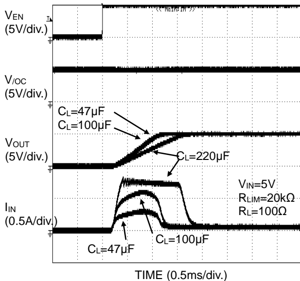
Figure 40. Inrush Current Response (BD2242G)
