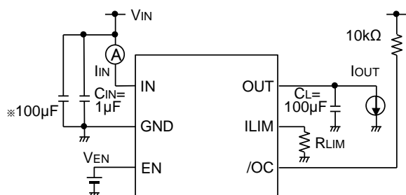
C. On-Resistance, Current Limit Threshold, /OC Delay Time
