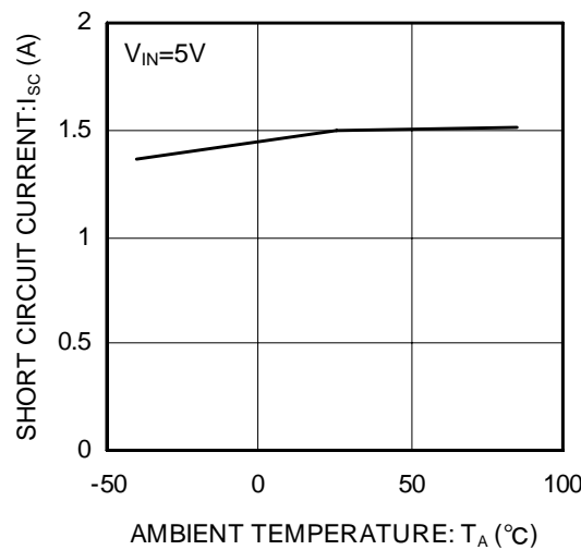
Figure 17. Short circuit current
