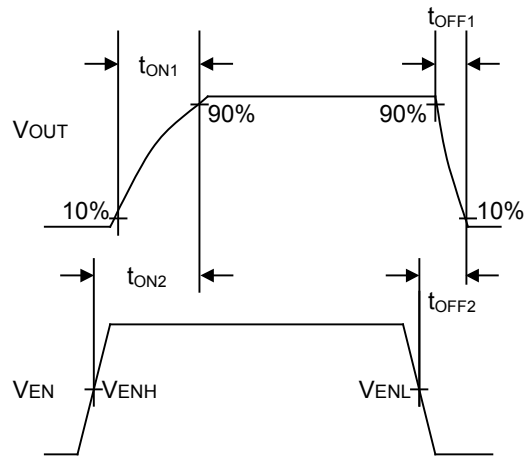
Figure 3. Timing Diagram(BD2066FJ)
