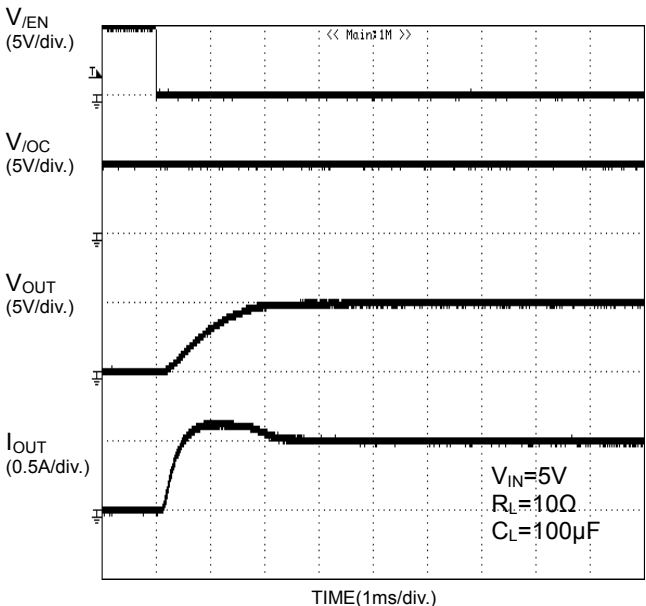
Figure 28. Output Rise Characteristic (BD2061AFJ)
