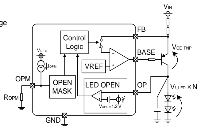
Figure 13. Disable LED Open Detection Function at Reduced-Voltage
