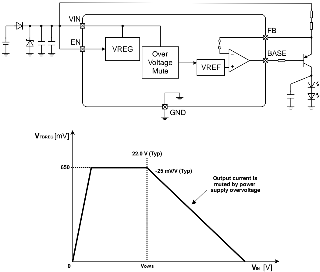
Figure 20. Overvoltage Mute Function (OVM)
