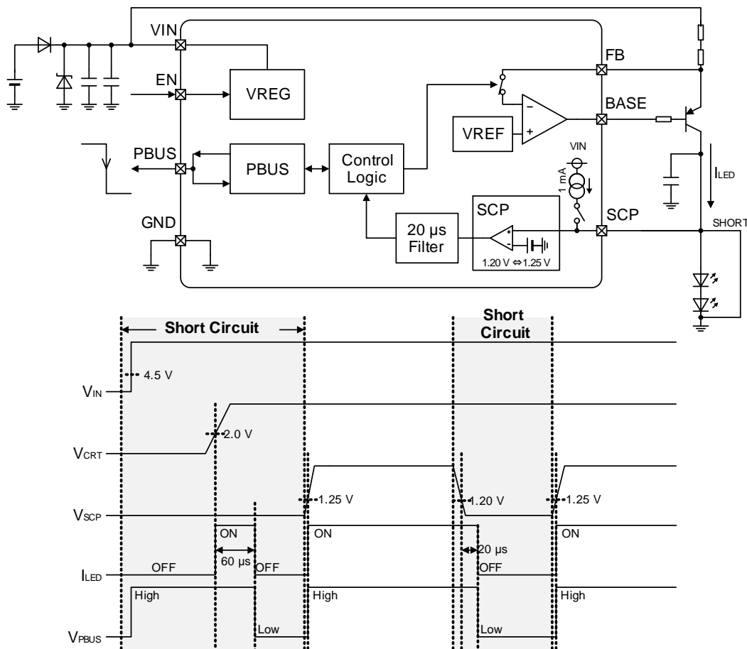
Figure 15. Short Circuit Protection (SCP)
