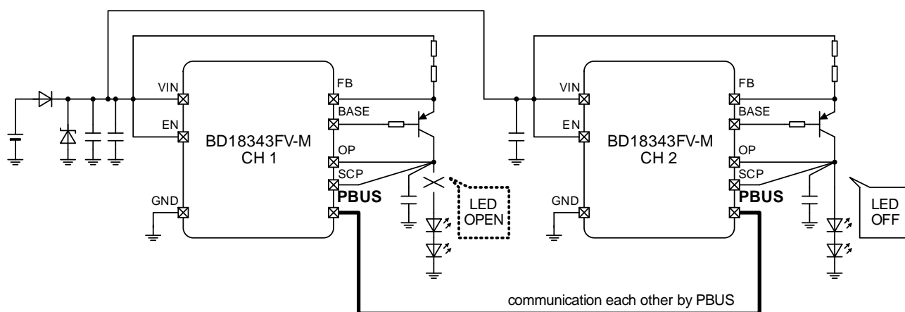
Figure 18. PBUS Function
