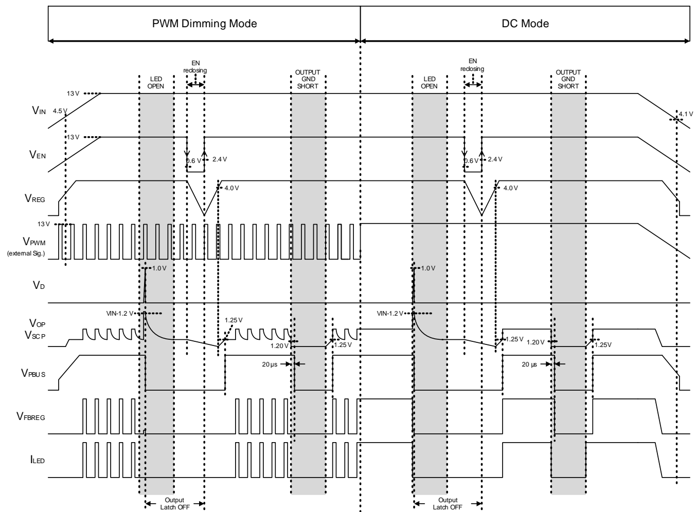
Figure 21. Timing Chart
