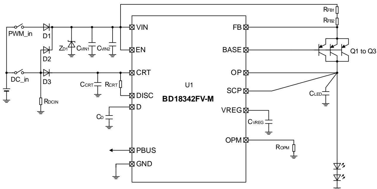
Figure 28. Application Example 3 (I_{LED} 524\text{ mA}, \text{LED white 2 strings, PWM ON Duty: } 10\% (\text{pulse width: } 0.334\text{ ms}), \text{PWM frequency: } 300\text{ Hz})
