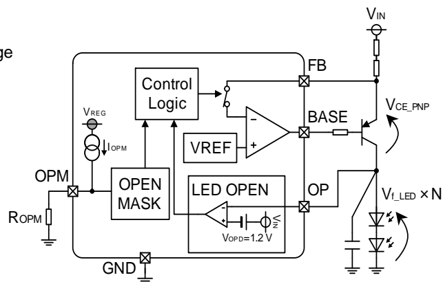
Figure 17. Disable LED Open Detection Function at Reduced-Voltage
