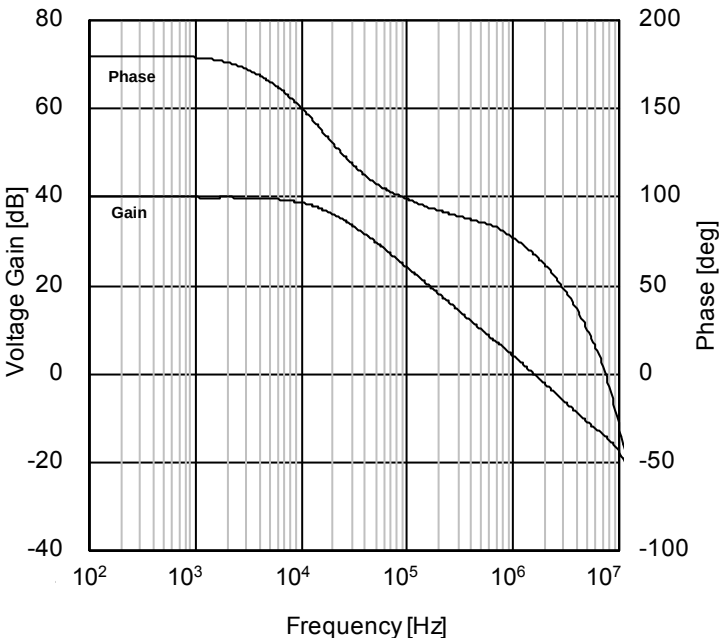
Figure 46. Voltage Gain · Phase vs Frequency ( V+=5V , R_L=2k\Omega , T_A=25^\circ C )
