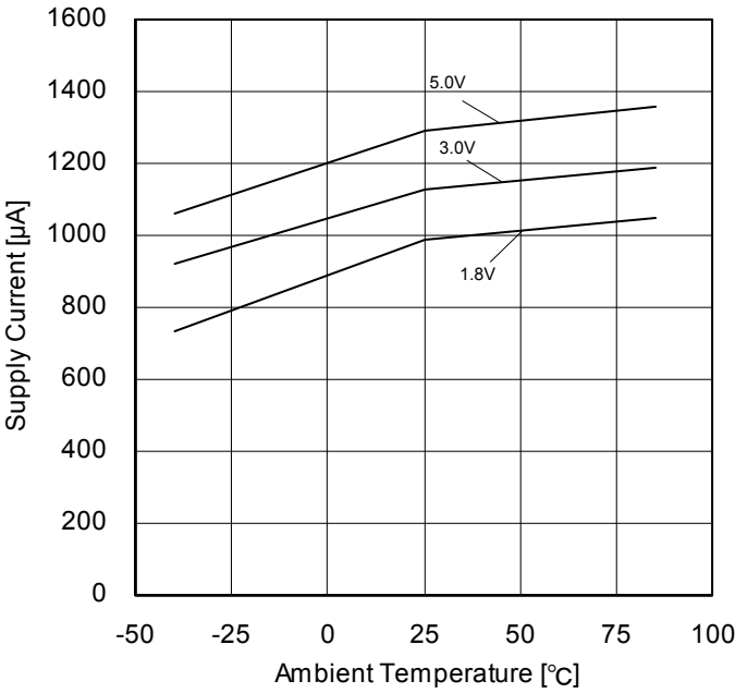
Figure 56. Supply Current vs Ambient Temperature
