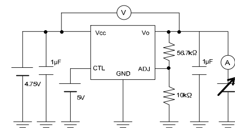
Measurement Circuit of Figure 9
