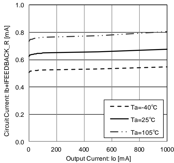
Figure 12. Circuit Current ( I_o=0\text{mA}\rightarrow1000\text{ mA} ) ( I_{FEEDBACK\_R}\doteq75\mu\text{A} )
