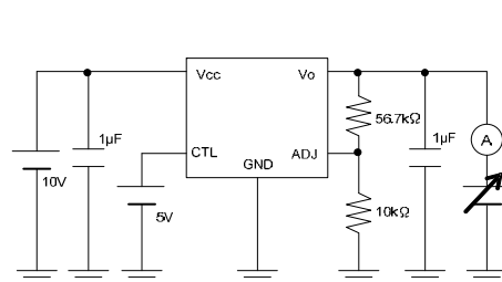
Measurement Circuit of Figure 8
