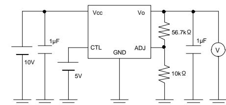
Measurement Circuit of Figure 15
