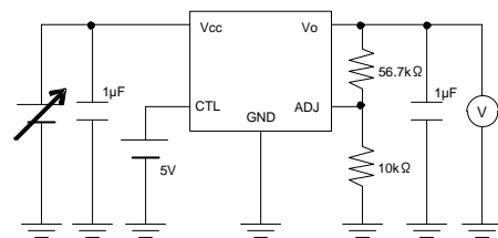
Measurement Circuit of Figure 6
