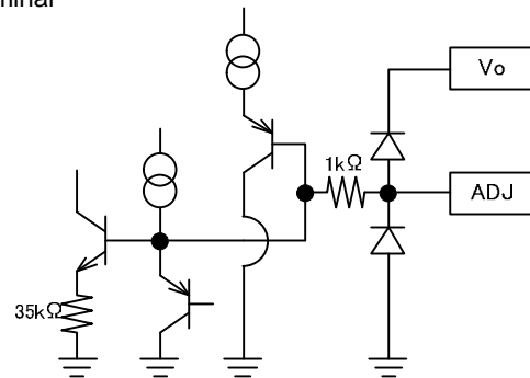
ADJ terminal
