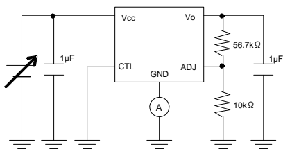
Measurement Circuit of Figure 5
