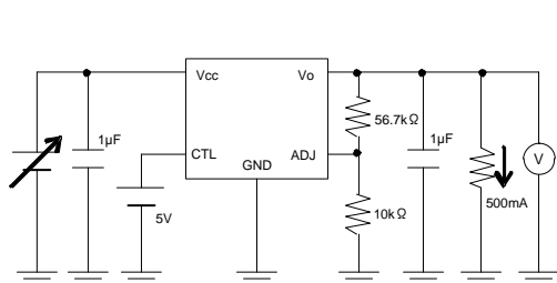
Measurement Circuit of Figure 7
