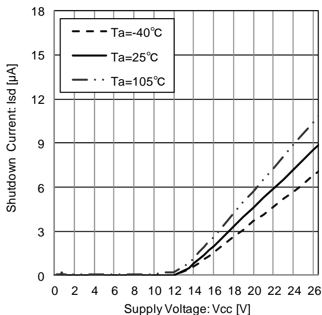
Figure 5. Shutdown Current
