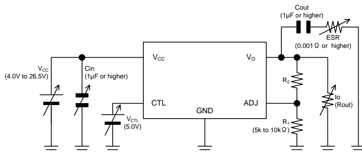
※Operation Note 11 Measurement circuit
