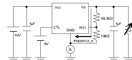
Measurement Circuit of Figure 12
