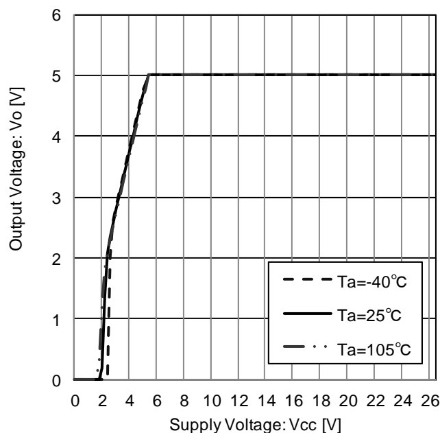
Figure 7. Line Regulation ( I_o=500mA )
