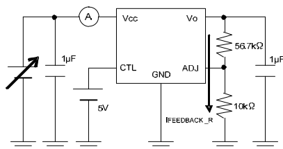
Measurement Circuit of Figure 4
