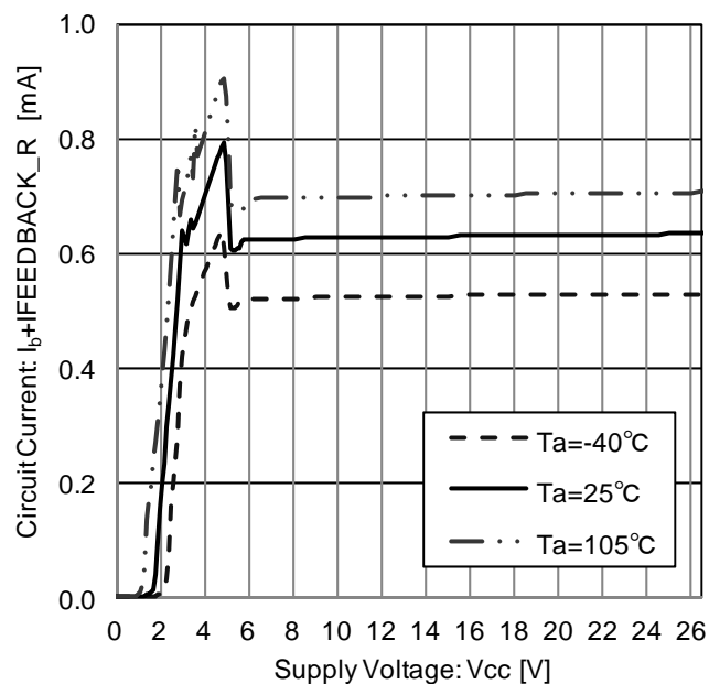
Figure 4. Circuit Current ( I_{FEEDBACK\_R} \approx 75\mu A )
