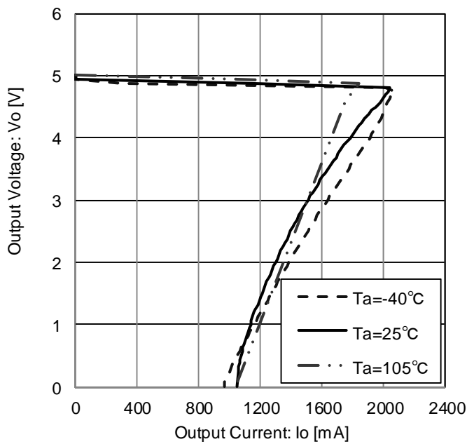
Figure 8. Load Regulation
