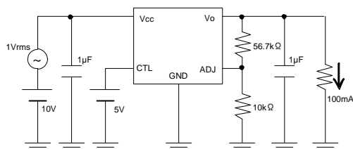
Measurement Circuit of Figure 10
