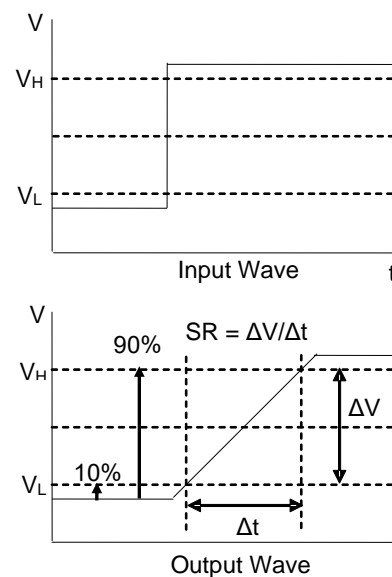
Figure 28. Slew Rate Input Output Wave
