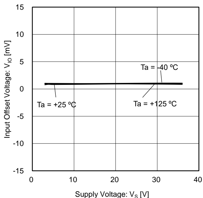
Figure 9. Input Offset Voltage vs Supply Voltage ( V_{ICM} = V_S / 2 , V_{OUT} = V_S / 2 )
