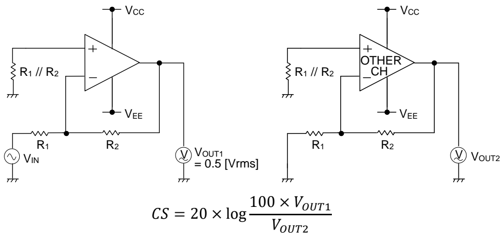
Figure 29. Test Circuit 3 (Channel Separation)
