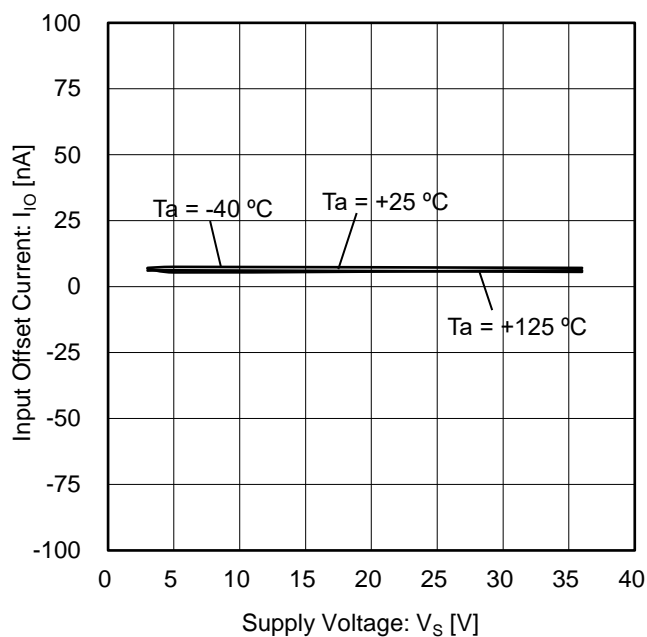
Figure 14. Input Offset Current vs Supply Voltage ( V_{1CM} = V_S / 2 , V_{OUT} = V_S / 2 )
