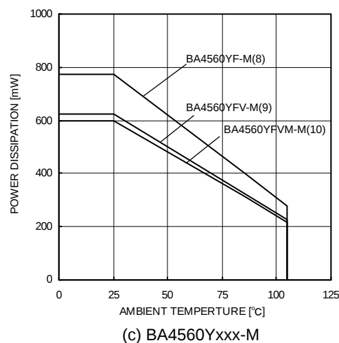
Figure 24. Thermal resistance and derating
