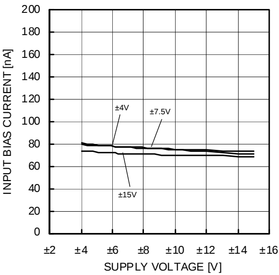
Figure 13. Input Bias Current - Ambient Temperature (Vicm=0V, OUT=0V)
