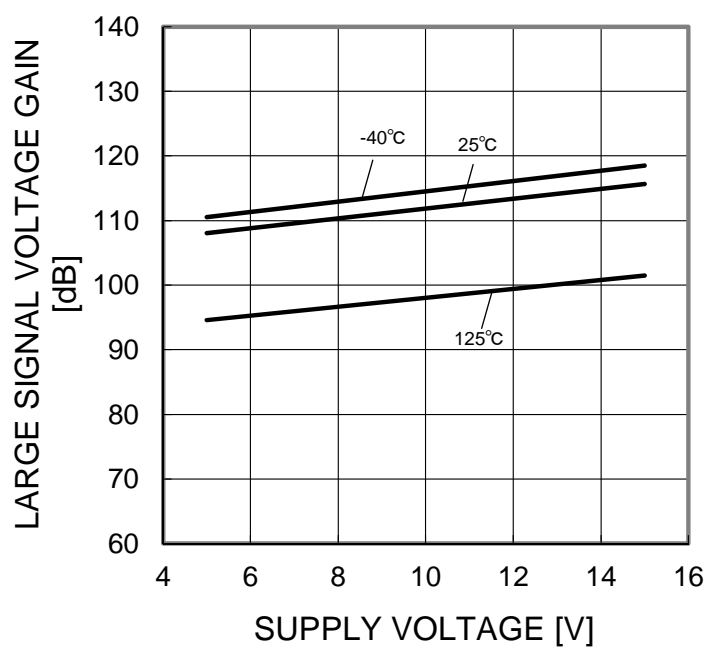
Figure 45. Large Signal Voltage Gain – Supply Voltage (R L =2kΩ)
