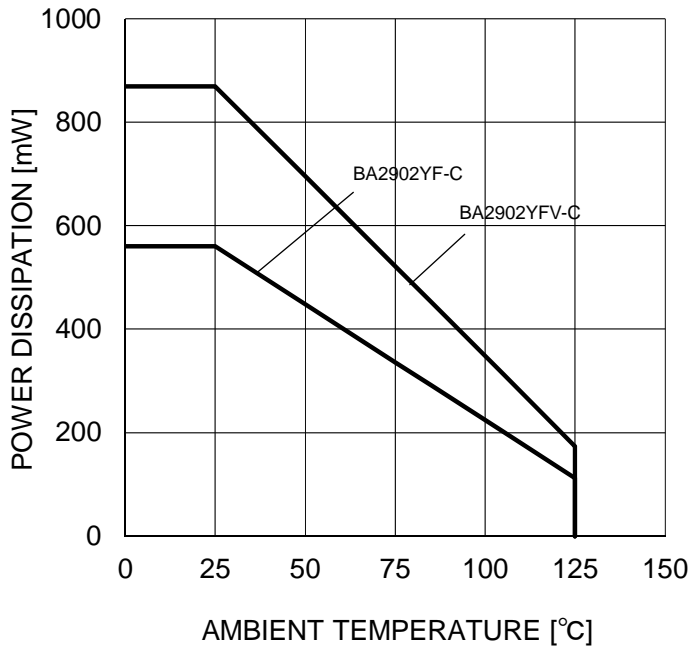
Figure 26. Derating Curve
