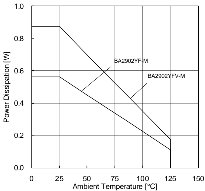
Figure 26. Derating Curve
