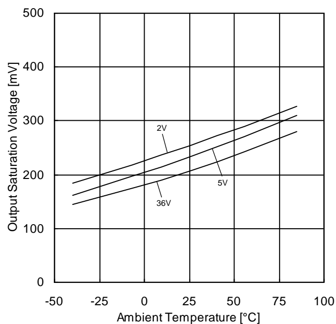
Figure 49. Output Saturation Voltage vs Ambient Temperature ( I_{OL}=4\text{mA} )
