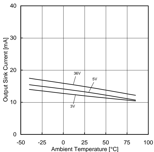
Figure 51. Output Sink Current vs Ambient Temperature ( OUT=1.5\text{V} )
