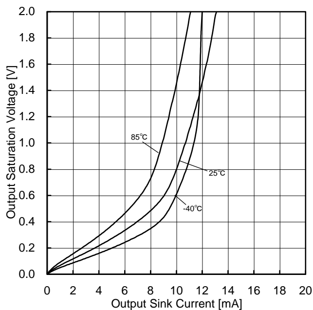
Figure 50. Output Saturation Voltage vs Output Sink Current ( V_{CC}=5\text{V} )
