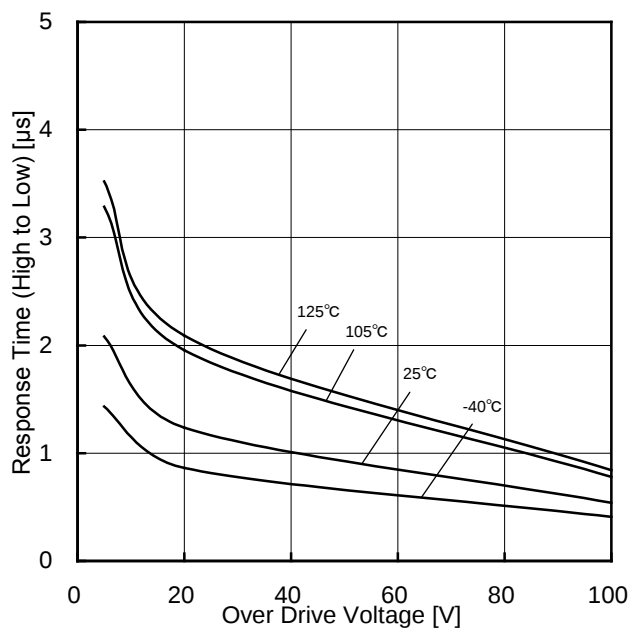
Figure 86. Response Time (High to Low) vs Over Drive Voltage ( V_{CC}=5\text{V} , V_{RL}=5\text{V} , R_L=5.1\text{k}\Omega )
