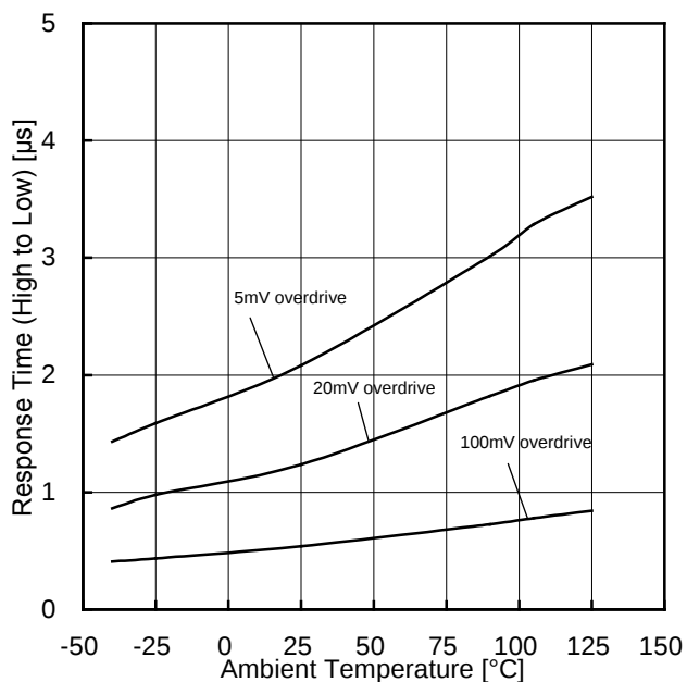
Figure 87. Response Time (High to Low) vs Ambient Temperature ( V_{CC}=5\text{V} , V_{RL}=5\text{V} , R_L=5.1\text{k}\Omega )
