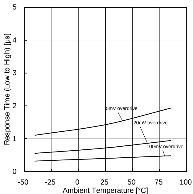
Figure 22. Response Time (Low to High) vs Ambient Temperature ( V_{\text{CC}}=5\text{V} , V_{\text{RL}}=5\text{V} , R_{\text{L}}=5.1\text{k}\Omega )
