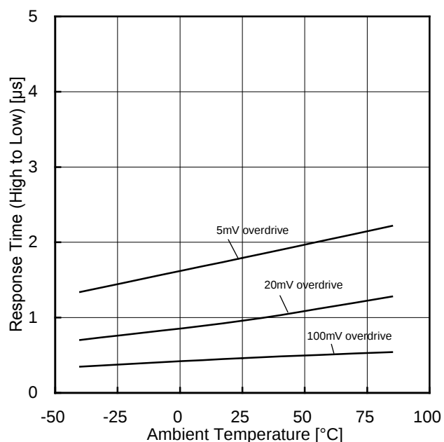
Figure 24. Response Time (High to Low) vs Ambient Temperature ( V_{\text{CC}}=5\text{V} , V_{\text{RL}}=5\text{V} , R_{\text{L}}=5.1\text{k}\Omega )
