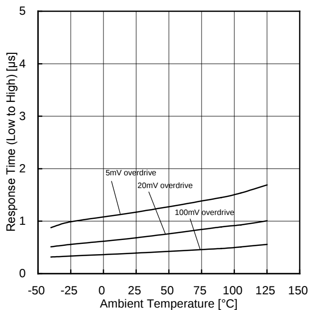
Figure 85. Response Time (Low to High) vs Ambient Temperature ( V_{CC}=5\text{V} , V_{RL}=5\text{V} , R_L=5.1\text{k}\Omega )
