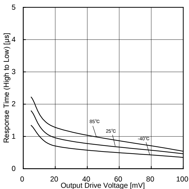
Figure 23. Response Time (High to Low) vs Over Drive Voltage ( V_{\text{CC}}=5\text{V} , V_{\text{RL}}=5\text{V} , R_{\text{L}}=5.1\text{k}\Omega )
