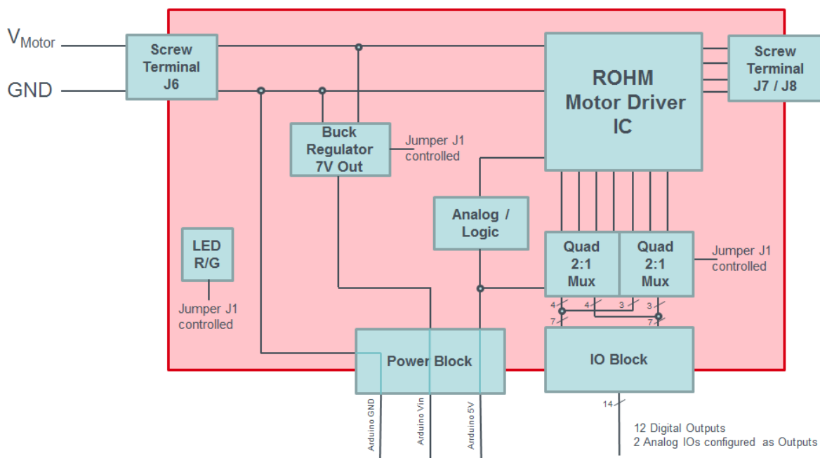
Figure 1: EVK Shield Block Diagram
