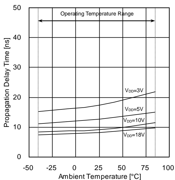
Figure 12. Propagation Delay Time t_{PHL} (IN→OUT) vs Ambient Temperature
