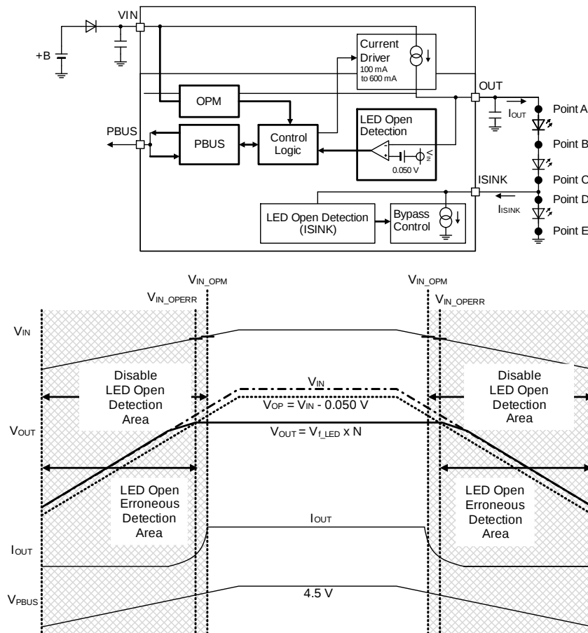
VIN Pin Disable LED Open Detection Voltage at Reduced-Voltage and LED Open Erroneous Detection Voltage at Reduced-Voltage
