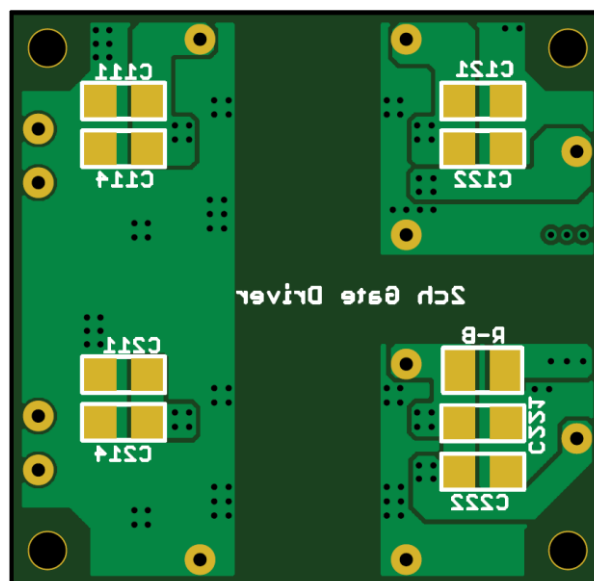
Bottom Layer with Pad and Silkscreen (Top View)
