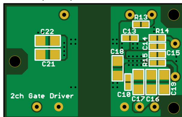
Silkscreen (Bottom)
