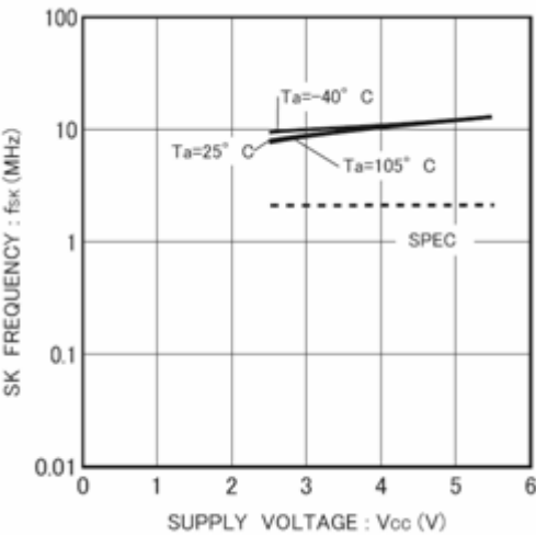
Figure 13. SK frequency f_{SK}
