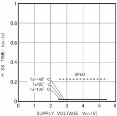
Figure 14. SK high time t_{SKH}
