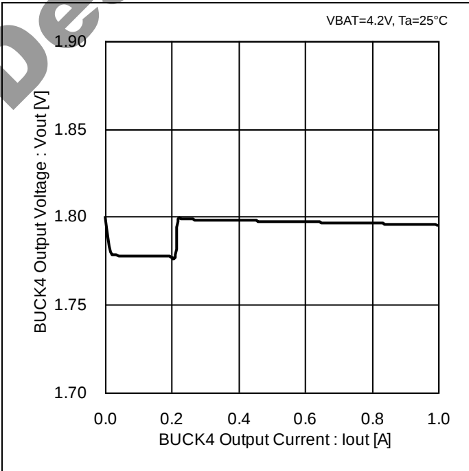
Figure 48. BUCK4 - Load Regulation (Auto Mode)
