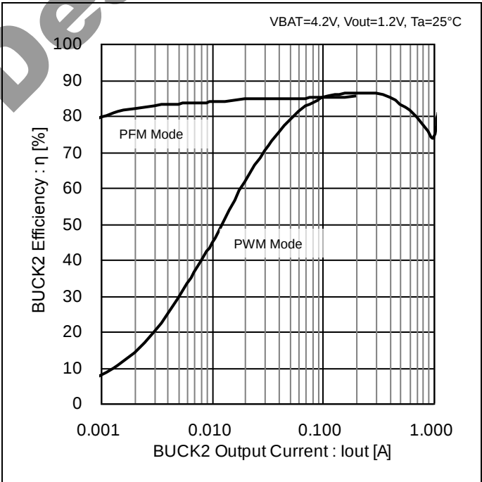
Figure 36. BUCK2 – Efficiency (PWM Mode / PFM Mode)
