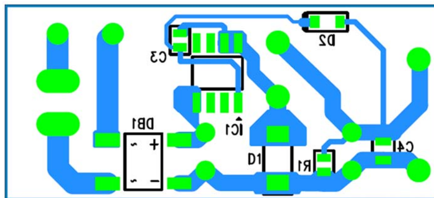
Figure 5. Bottom Layout (Top view)
