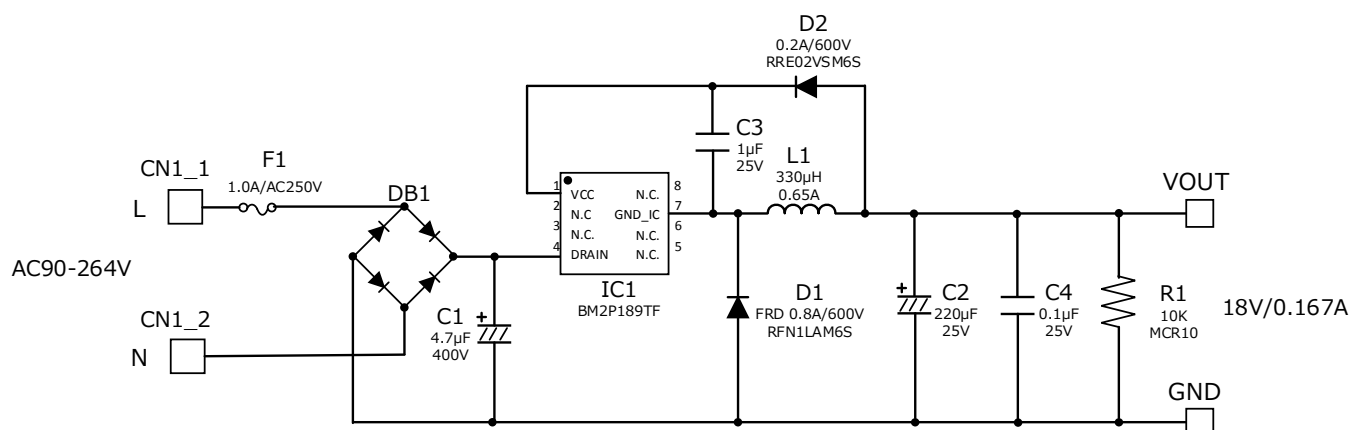
Figure 3. BM2P189TF-EVK-001 Schematics
