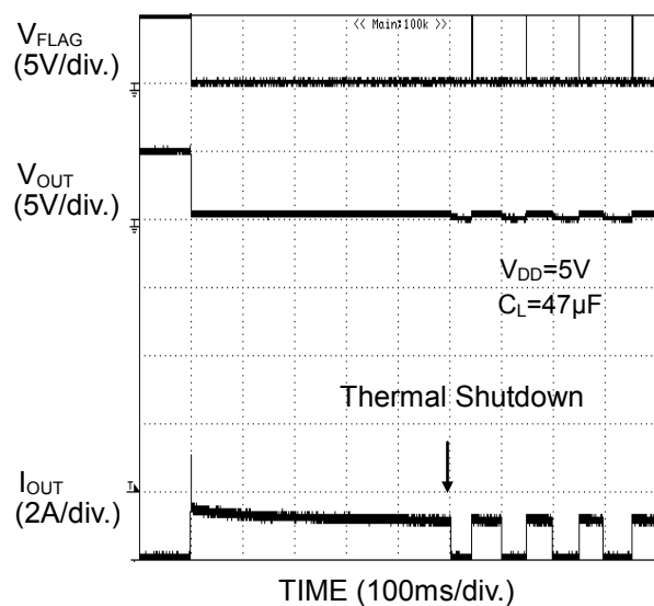
Figure 59. Over-Current Response 1Ω Load Connected at Enable (BD6516F)
