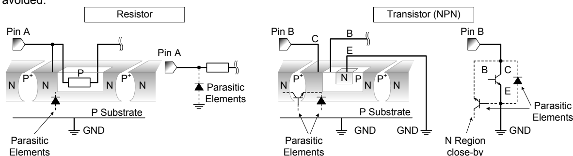
Figure 63. Example of monolithic IC structure
