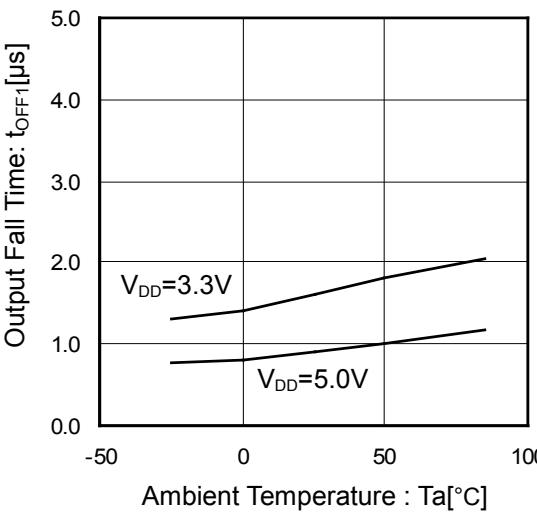
Figure 18. Output Fall Time vs Ambient Temperature
