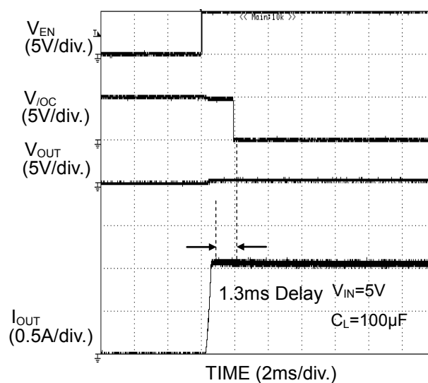
Figure 58. Over-Current Response Enable to 1Ω Short Circuit (BD2052AFJ)
