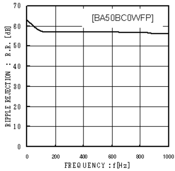
Fig.9 Ripple Rejection
